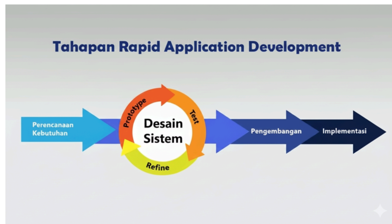
Gambar 2.4 RAD Model
